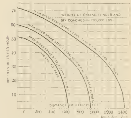
FIG. 7. SOME REMARKABLY GOOD STOPS AT 70, 60, AND 50 MILES PER HOUR, SHOWING POSSIBILITY OF HIGH-SPEED BRAKES.
